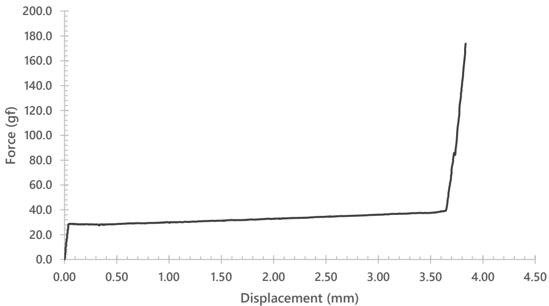
HMX Lulu Silent (Upstroke)
